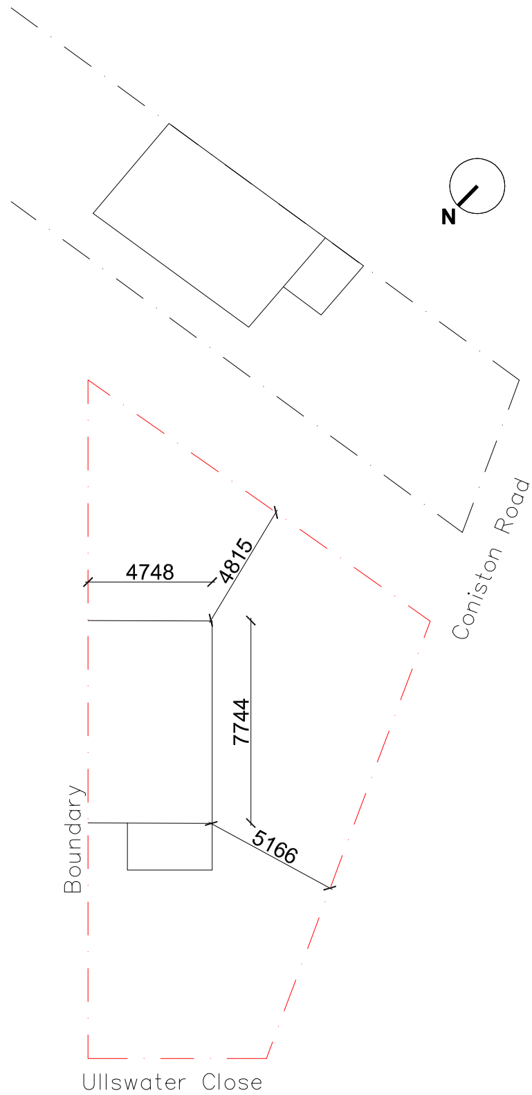
Existing Site plan scale 1:200
