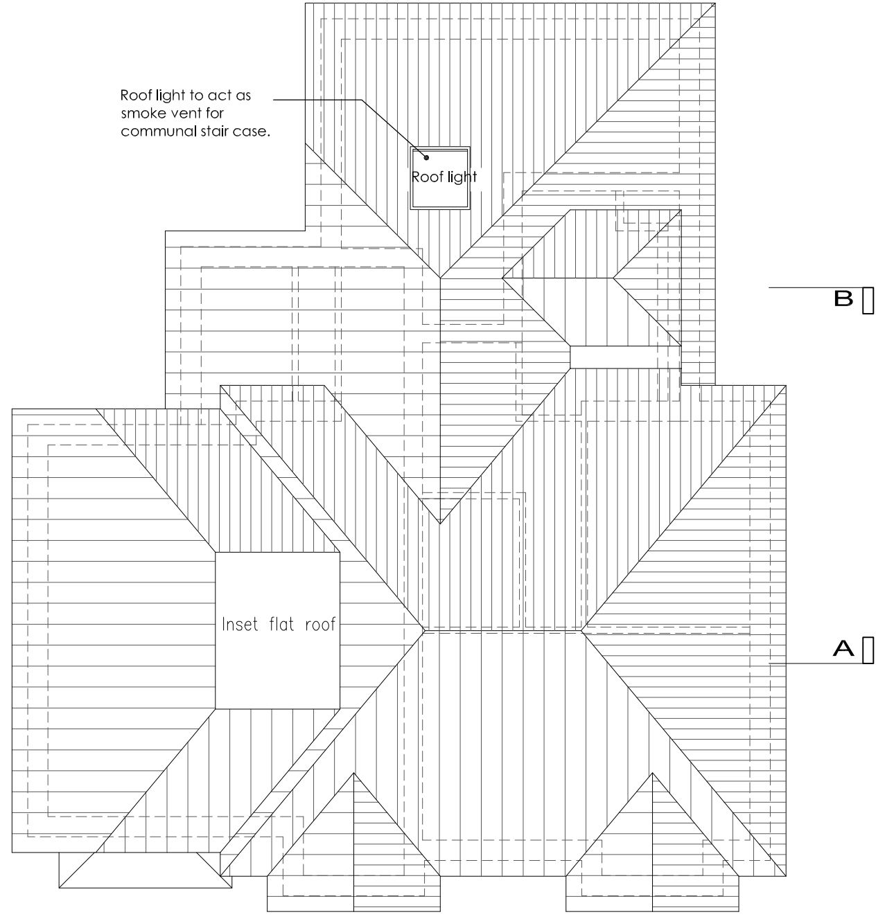
ROOF PLAN
